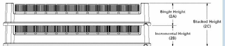
▲ Figure 2: Stacked Tray View
