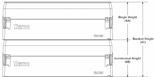
▲ Figure 4: Stacked Rack View
